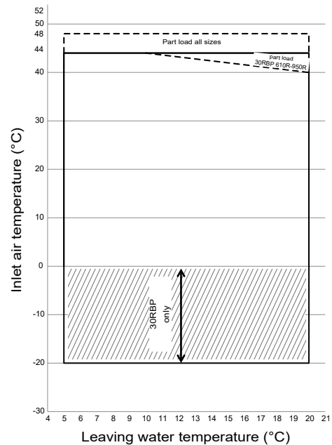
Operating range - Unit option 15LS 30RB/RBP 170R-950R option 15LS
