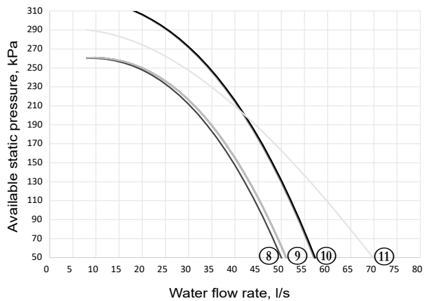
Sizes 620R - 1040R
