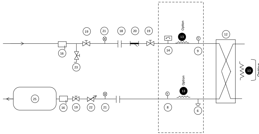
Typical hydraulic circuit diagram without hydraulic module
