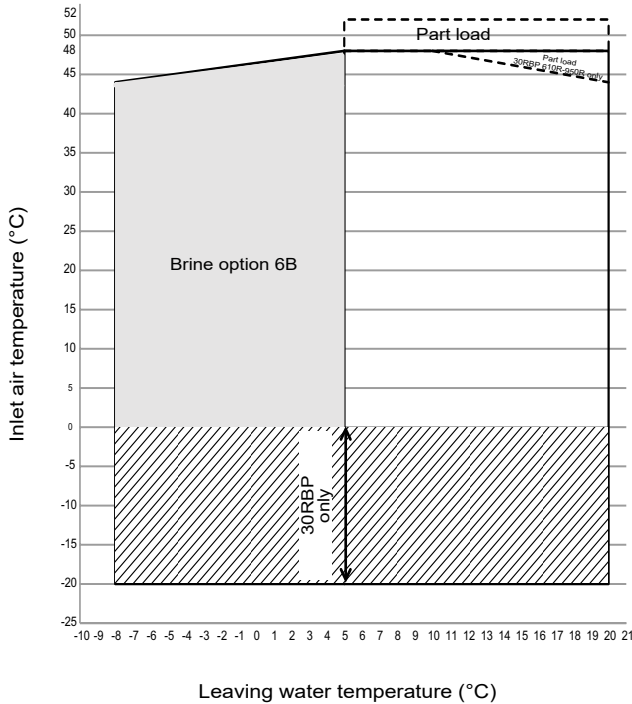
Operating range Standard unit
