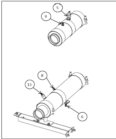
Figure 2: Hydraulic connections with hydraulic module
