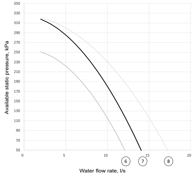
Sizes 410R - 550R
